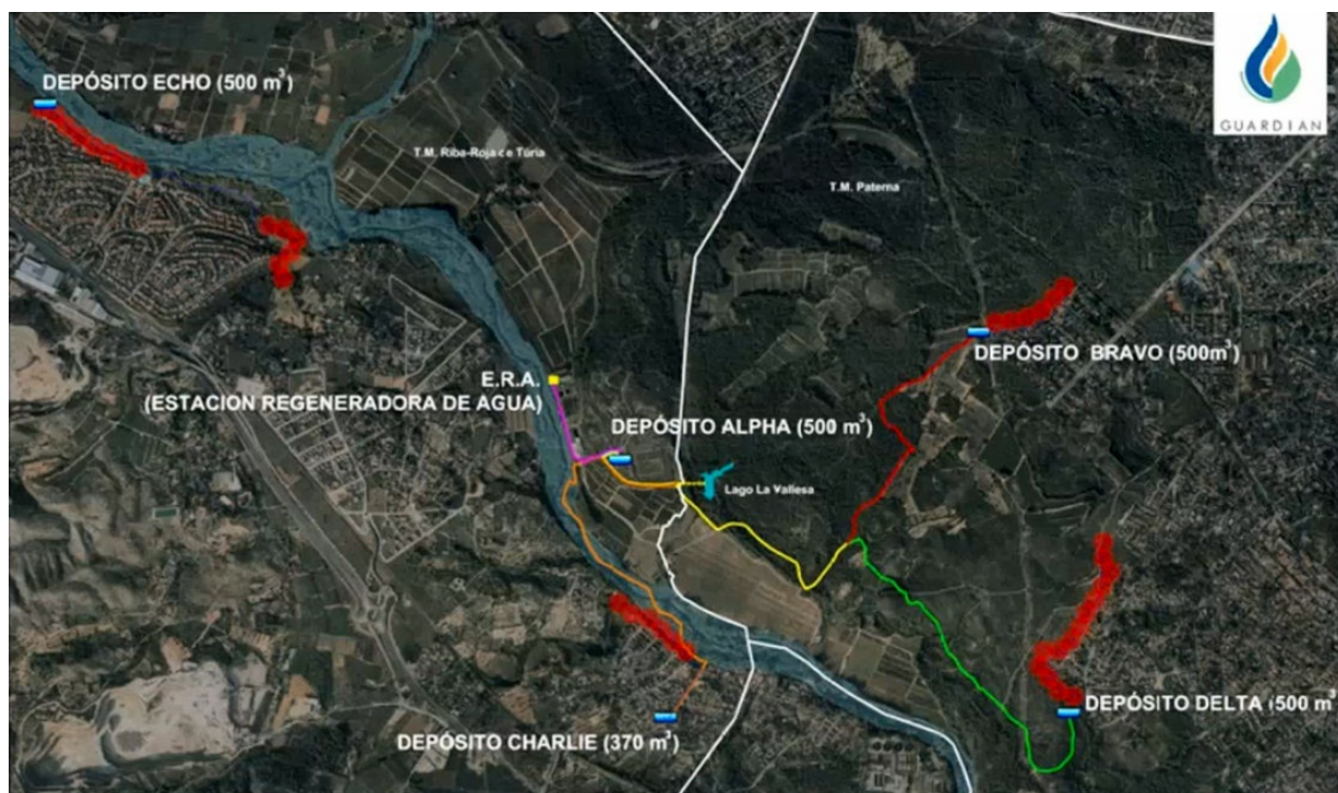
Figure 2. GUARDIAN hydraulic infrastructure scheme (northerly oriented). Spanish-English translation key: ERA – Estación Regeneradora de agua = WRP – Water Reclamation Plant; Depósito = Tank; Lago La Vallesa = La Vallesa reservoir. Recycled water is conveyed from the WRP to the main tank (Alpha) through a pressure pipe. Water from Alpha can then be pumped either to Bravo tank (to protect “Cañada Norte” settlement), or to Delta tank (to protect “Cañada Sur” settlement), or to Charlie tank (to protect “Els Pous” settlement) or to “la Vallesa” wetland (to contribute to increase ecosystems’ quality). In the northwest corner, the Echo tank is also under construction to deliver water to the “Masia Traver” settlement. Water to be accumulated in Echo will be conveyed through the existing irrigation ditch. Red zones are the areas where the water canyons will be deployed.
